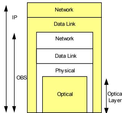
Figure 3. IP-over-OBS hierarchical layered architecture.
