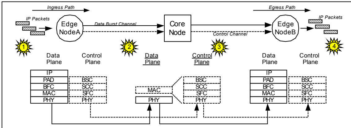
Figure 7. Layered view of an OBS network.
