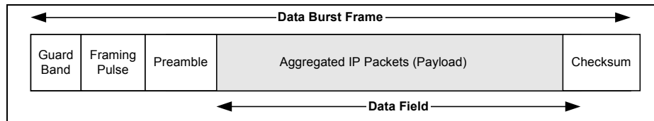
Figure 5. OBS framing structure of the data burst.
