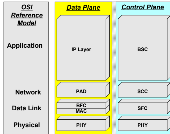
Figure 4. IP over OBS layered architecture.
