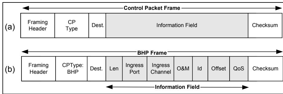
Figure 6. OBS framing structure of the control packet; (a) a generic control packet frame, (b) BHP frame
